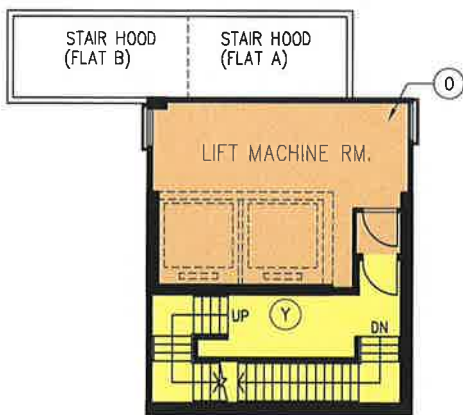
LIFT MACHINE RM. FLOOR PLAN AT LEVEL 102.87
