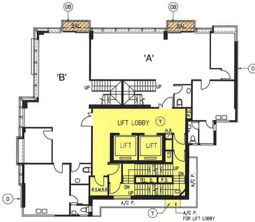
DUPLEX LOWER FLOOR PLAN (28th FLOOR)
