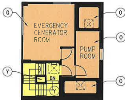
EMERGENCY GENERATOR ROOM FLOOR PLAN AT LEVEL 105.67
